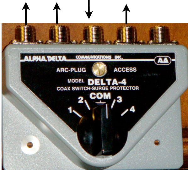
SWITCH 2
